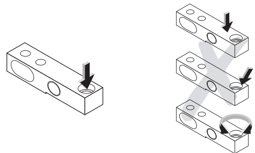
Right mounting
