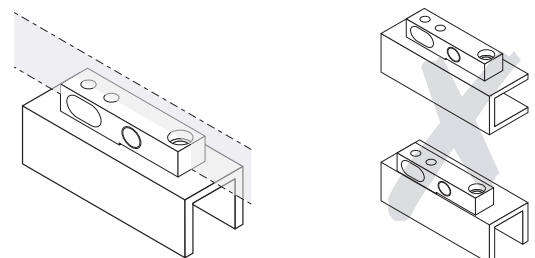
Right mounting
